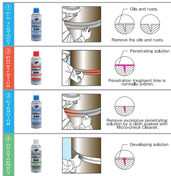
Crack detection test at heat seal package.
